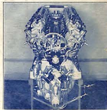
Control-end view of the 550-600 H. P. Directly Reversible Maybach motor.
