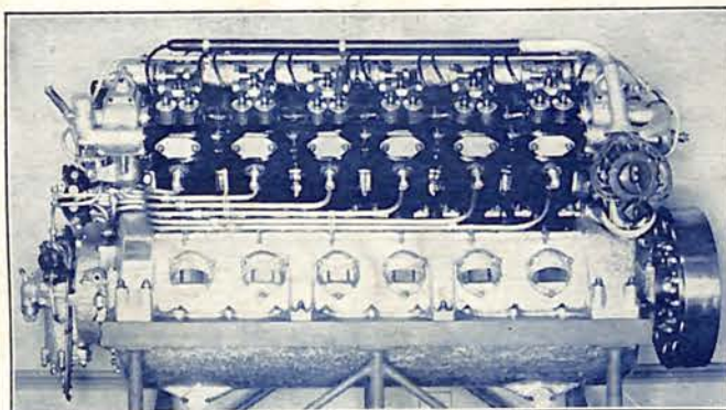
Side view of the famous Maybach type V, L-2 Directly Reversible motor, five of which provide power for the Graf Zeppelin. Full details on request.
