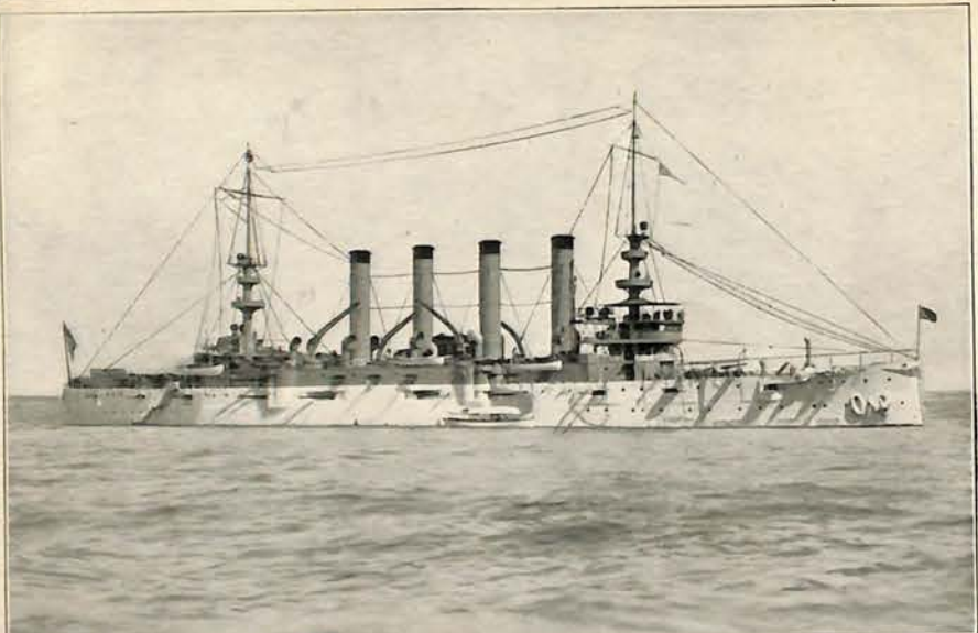
No. 5030.—U. S. PROTECTED CRUISER "CHARLESTON." 600 officers and men. Displacement, 9,500 tons. Speed, 22 knots. Bunker capacity, 1,500 tons. Armor: Belt, 4 in.; topsides, 4 in.; deck, flat 2 in., slopes 3 in. Complement, 564. Length, 424 ft.
